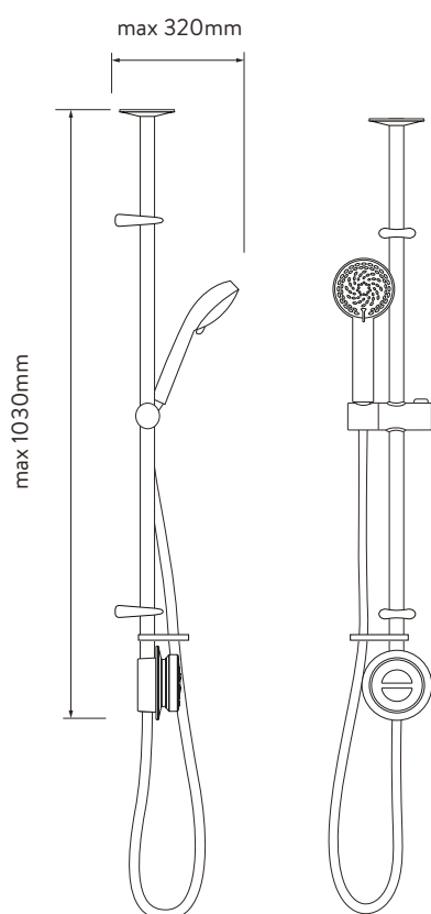
AQUALISA SMARTVALVE™
